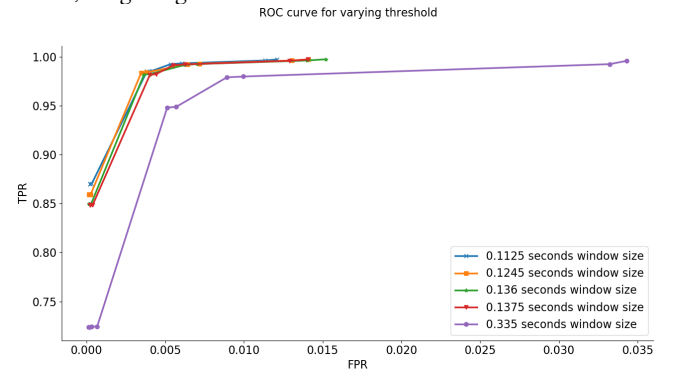
Figure 5: ROC curve of varying thresholds for different window sizes using fuzzy attack dataset
