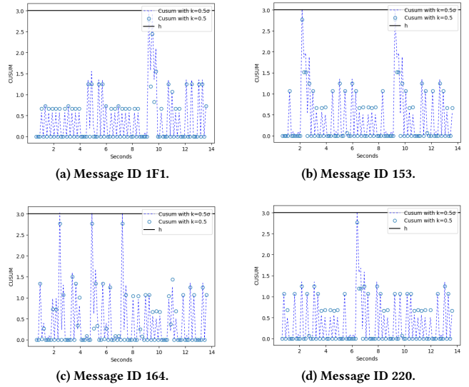
Figure 1: Plots of CUSUM algorithm with reference parameter k fixed to 0.5 and varied at (0.5 * \sigma) for attack free dataset \theta = \theta_0 , the in-control ARL_0 is the expected number of samples before a false alarm, and \theta = \theta_1 , the out-of-control ARL_1 is the expected number of samples before a shift in the mean is detected. A specific value is required for ARL_0 while we aim to minimize ARL_1 value over a range of process shifts. We also evaluate the performance by calculating the true positive rate (TPR) and the false positive rate (FPR) after measuring the number of true negative (TN), true positive, false positive (FP), and false negative (FN).
