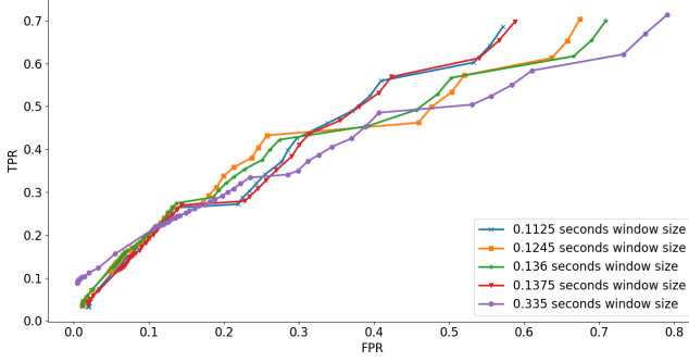
Figure 2: Adaptive CUSUM Algorithm performance on varying thresholds for different window sizes using RPM dataset
