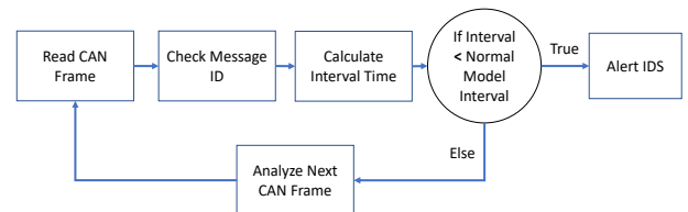
Figure 2: Every CAN message is read and its ID captured. The time interval from current to previous message with the same ID is calculated and compared to the normal model timing interval for that message. If the interval time is less than normal, the IDS will indicate an anomaly and the IDS sends an alert.
