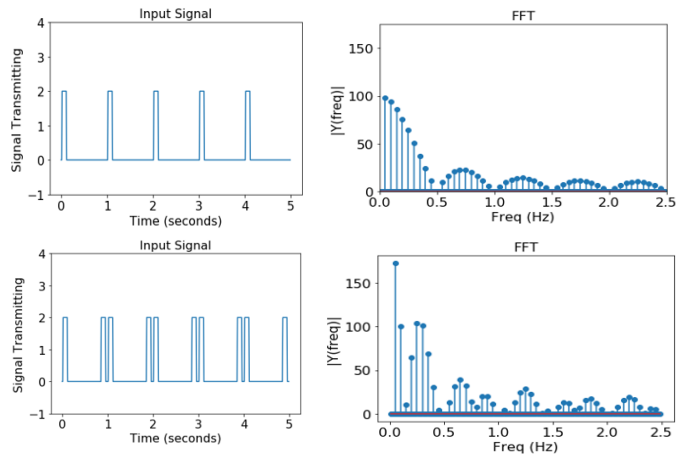
Figure 7: As the message rate doubles during injection attack, the magnitudes of certain frequency peaks will increase.
